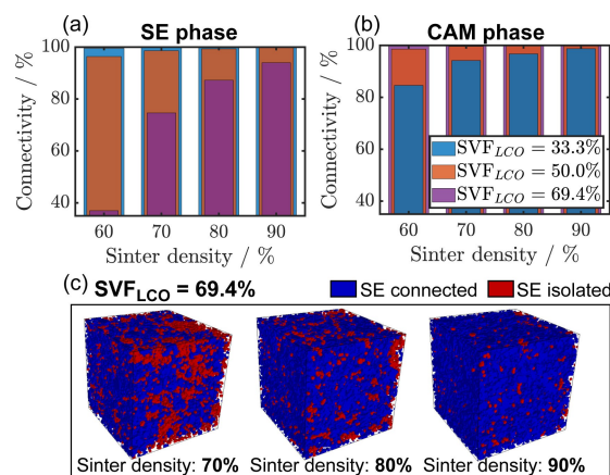
Figure 6. Influence of the density after sintering on the connectivity in the (a) SE phase and (b) CAM phase for SVF_{LCO} = 33.3, 50.0 and 69.4\% . (c) The influence of the density after sintering on the connectivity in the SE phase for the 3D composite cathode structure with SVF_{LCO} = 69.4\% . The mean initial particle diameters were constant at d_{CAM} = 2.00 \mu m and d_{SE} = 1.41 \mu m .
