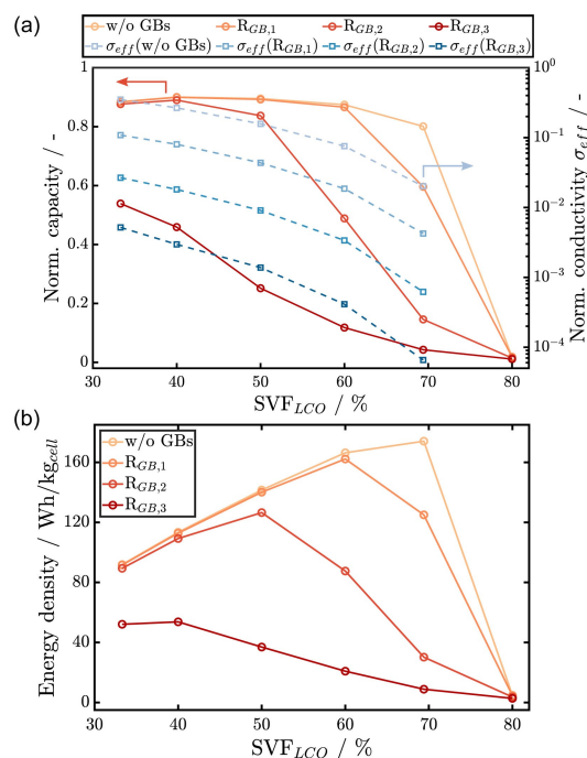
Figure 4. Influence of the grain boundary resistance on the (a) effective ionic conductivity and normalized capacity and (b) energy density. R_{\text{GB},1} = 3.6 \cdot 10^{-2}\ \Omega\text{cm}^2 , R_{\text{GB},2} = 3.6 \cdot 10^{-1}\ \Omega\text{cm}^2 , R_{\text{GB},3} = 3.6\ \Omega\text{cm}^2 . The density after sintering and mean initial particle diameters were constant at \rho_s = 93.1\% , d_{\text{CAM}} = 2.00\ \mu\text{m} and d_{\text{SE}} = 1.41\ \mu\text{m} . The discharge simulations were conducted at a current density of 1\ \text{mA/cm}^2 .
